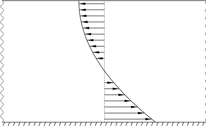
FIGURE 10. The azimuthal velocity profile (4.2) of a rimming flow.
